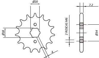
HB03.4_428 XL125Z / XL185SZ TYPE JAPANESE
