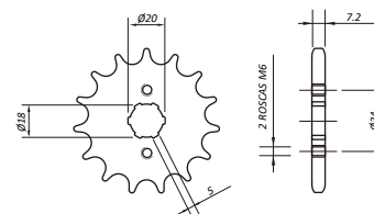
HB02.2_428 XL250 BAJA JIALING 125
