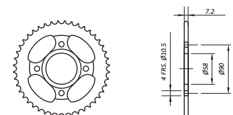
HA04.1_428 XL125SZ XL185SZ WITHOUT ANEL
