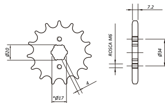
HB03.2_428 XL125 S TYPE BRASIL
