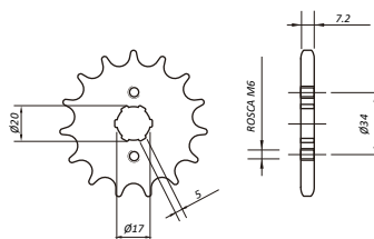
HB03.1_428 NXR125 / NXR150
