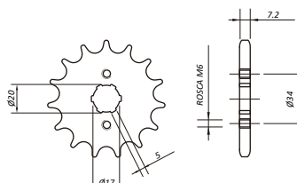
HB03.1_428 NXR125 / NXR150
