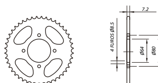
YA01.5_428 RX100 YB125E YBR125E
