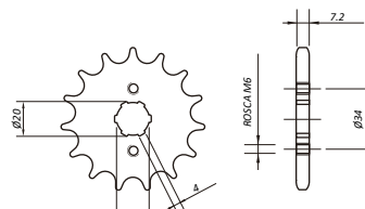
HB03.2_428 XL125 S TYPE BRASIL
