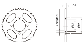
YA01.5_428 RX100 YBR125E
