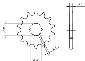
SB02.2_428 GN125 GN125H
