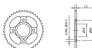
HA04.1_428 XL125SZ XL185SZ WITHOUT ANEL
