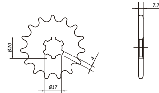
YB02.1_428 DT175 E DT175 K
