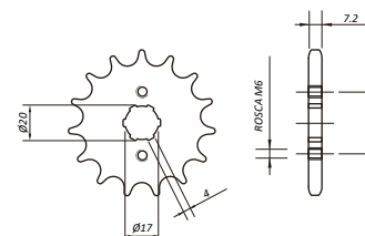
HB03.2_428 XL125 S TYPE BRASIL
