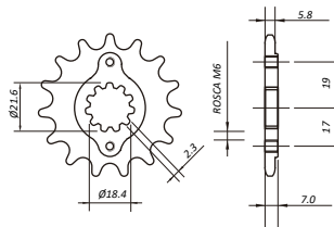
HB17.1_520 CBX250 XR250 TORNADO
