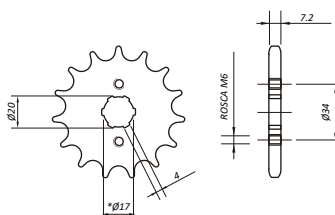
HB03.2_428 XL125 TYPE BRASIL
