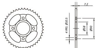
HA04.1_428 XL125SZ XL185SZ WITHOUT ANEL
