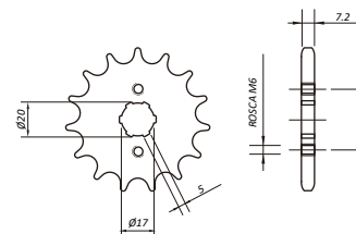
HB03.1_428 NXR125 / NXR150
