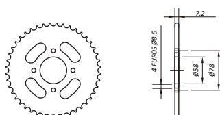
SA02.1_428 GN125 EN125 GN125H
