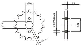
HB03.4_428 XL125SZ / XL185SZ TYPE JAPANESE
