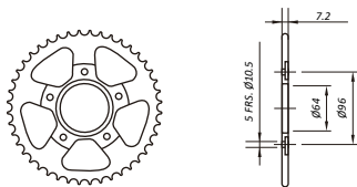
HA12.4_428 XLR125 BRASIL XLR125 JAPANESE
